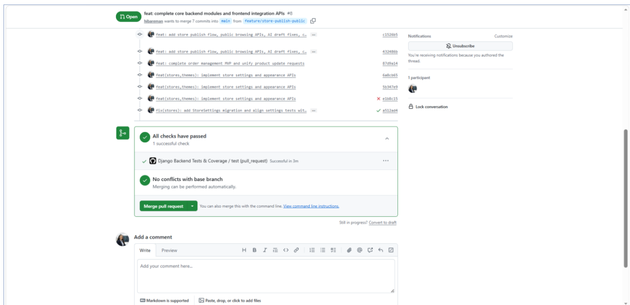
Figure 2.7 Merge Operations 2
